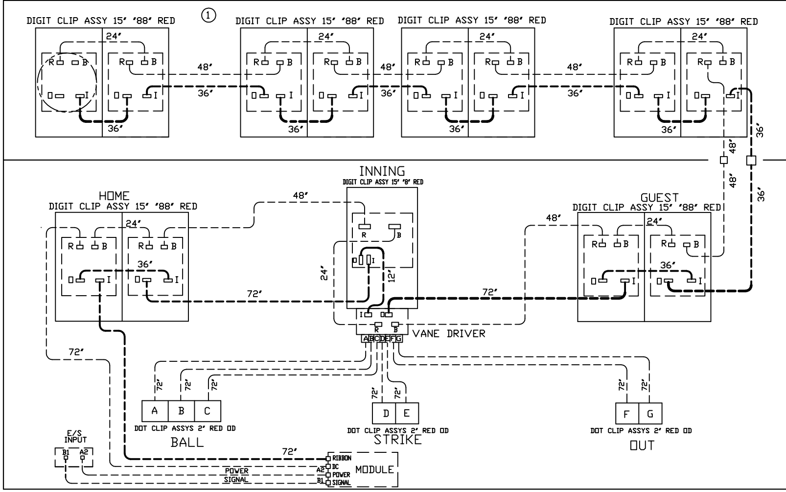
FRONT VIEW OF PANEL
