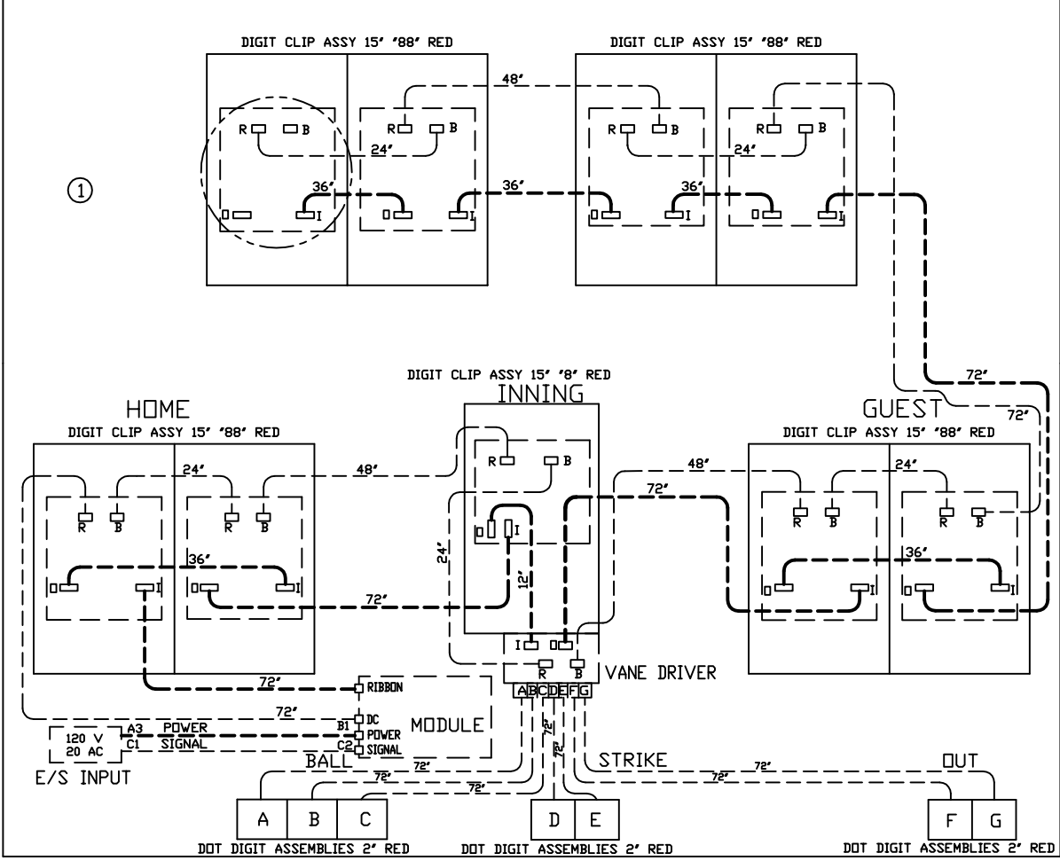
FRONT VIEW OF SCOREBOARD
