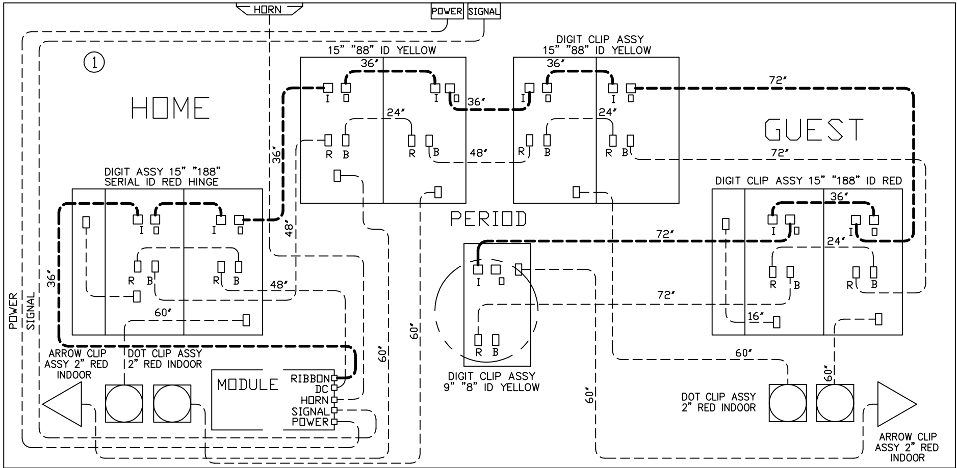
FRONT VIEW OF PANEL
