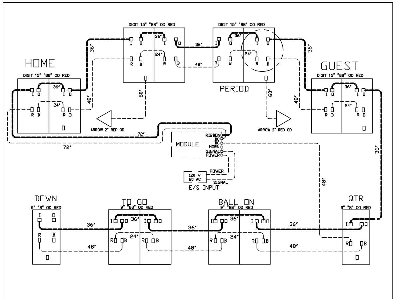
FRONT VIEW OF SCOREBOARD
