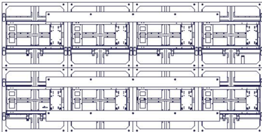
8810 Rear View showing J-channel Layout)
